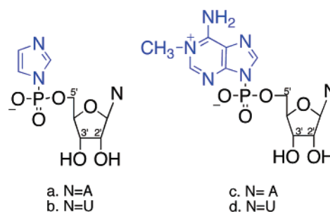
Figure 1. Activated monomers of nucleotides: (a) 5'-phosphorimidazolide of adenosine (ImpA), (b) 5'-phosphorimidazolide of uridine (ImpU), (c) adenosine 5'-phosphoro-1-methyladenine (MeadpA), (d) uridine 5'-phosphoro-1-methyladenine (MeadpU).
